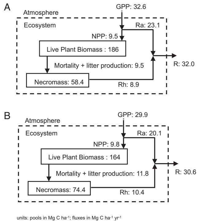
Fig. 4. Carbon pools (boxes, \text{MgC ha}^{-1} ) and fluxes (arrows, \text{MgC}\cdot\text{ha}^{-1}\cdot\text{yr}^{-1} ): (A) before logging; and (B) for the 3-y period following logging (Table S3). Carbon pools include live plant biomass ( 186\text{ MgC ha}^{-1} ) (34), necromass ( 58.4\text{ MgC ha}^{-1} ) (53), and soil mineral carbon ( 71\text{ MgC ha}^{-1} ) (54).
